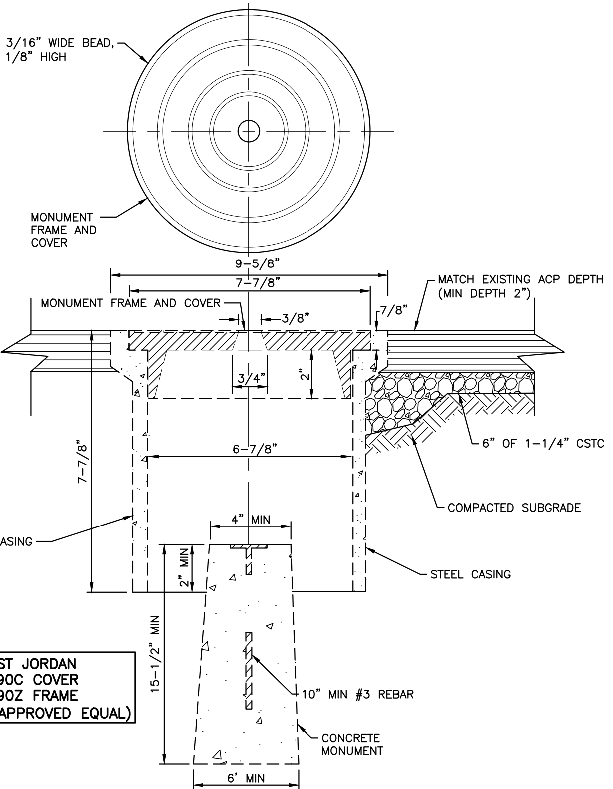
STANDARD CASED CONCRETE MONUMENT
